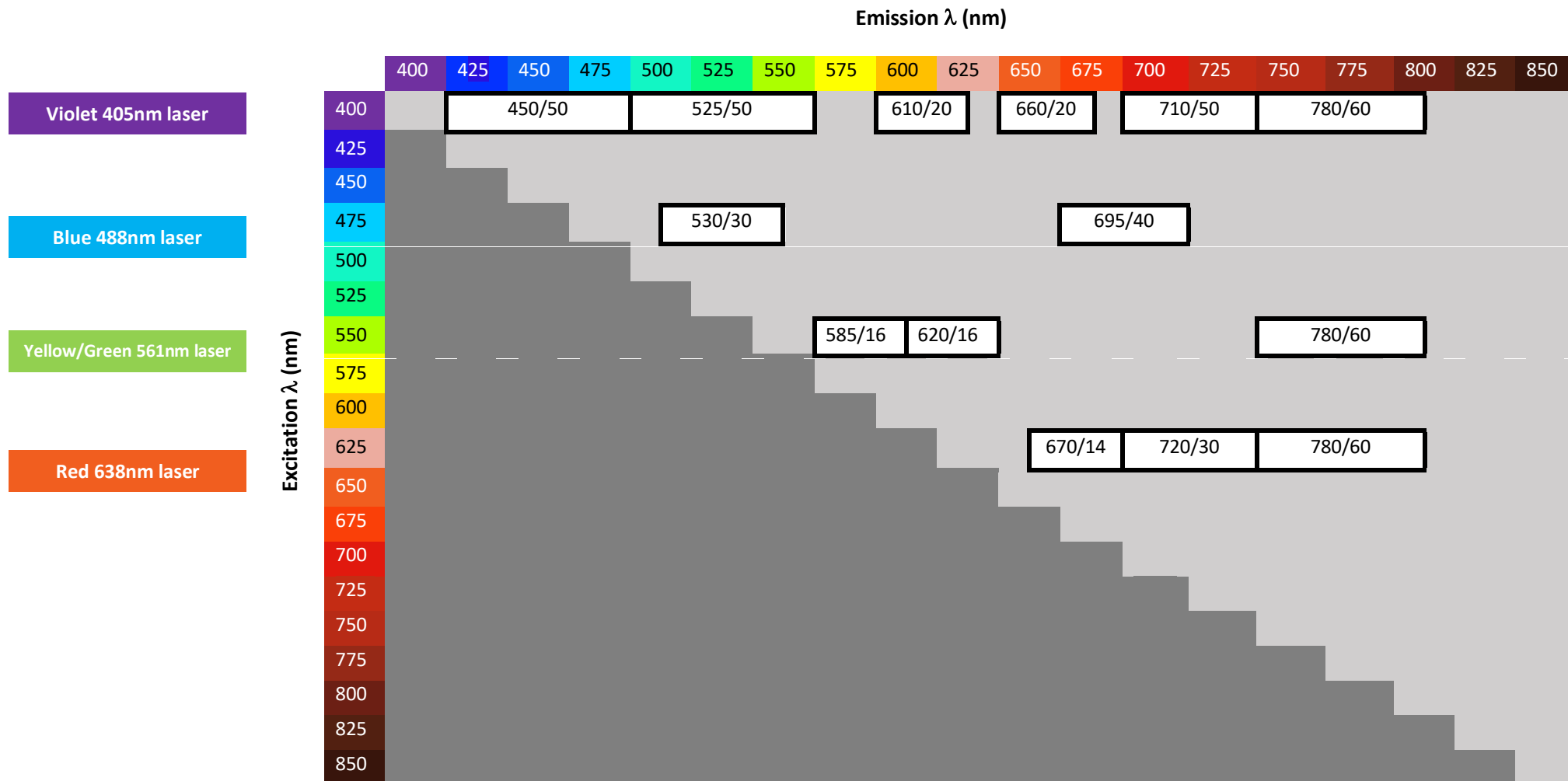
Greatest spectral spill-over and spread from neighbouring detectors for a given wavelength
